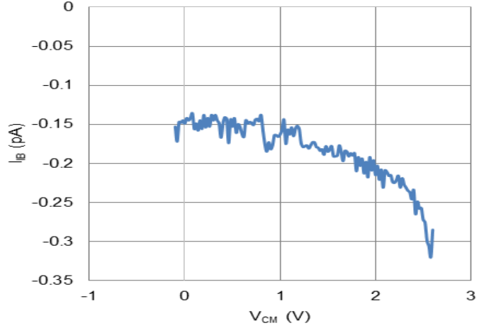
Figure 6. Input Offset Current vs. V_{CM} at V_S = 2.5\text{ V}
