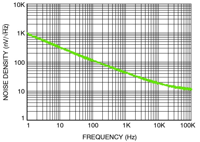
Figure 24. Voltage Noise Density vs. Frequency
