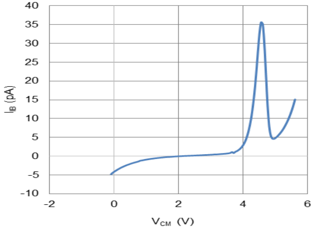
Figure 5. Input Bias Current vs. V_{CM} at V_S = 5.5\text{ V}
